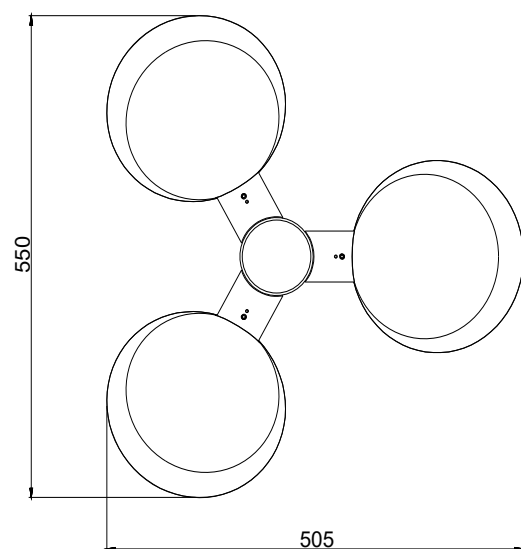
TRIPLE HEAD CONFIGURATION TOP VIEW (scale 1:5)
