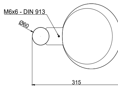
SINGLE HEAD CONFIGURATION TOP VIEW (scale 1:5)
