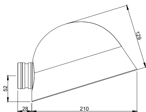
SIDE VIEW (scale 1:2)
