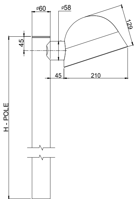
SIDE VIEW (scale 1:5)
