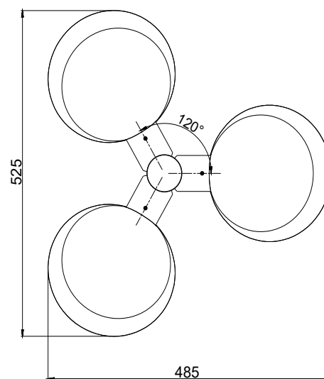
TRIPLE HEAD CONFIGURATION TOP VIEW (scale 1:5)
