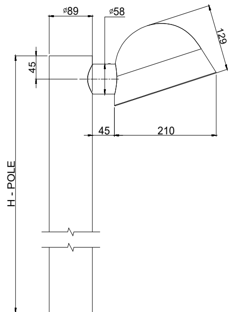
SIDE VIEW (scale 1:5)
